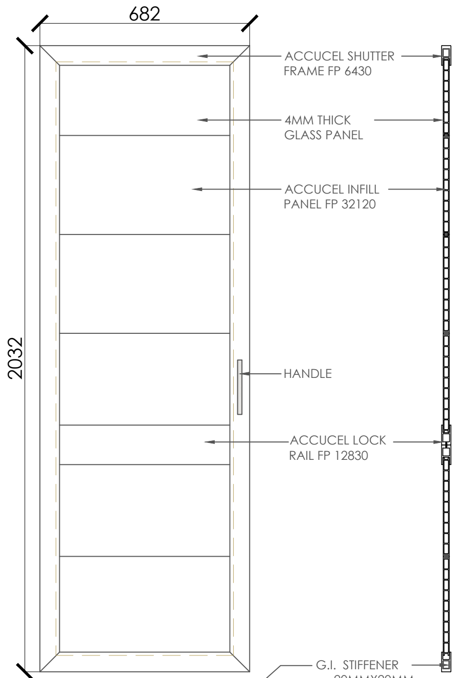
FRONT VIEW DOOR SHUTTER SECTION
